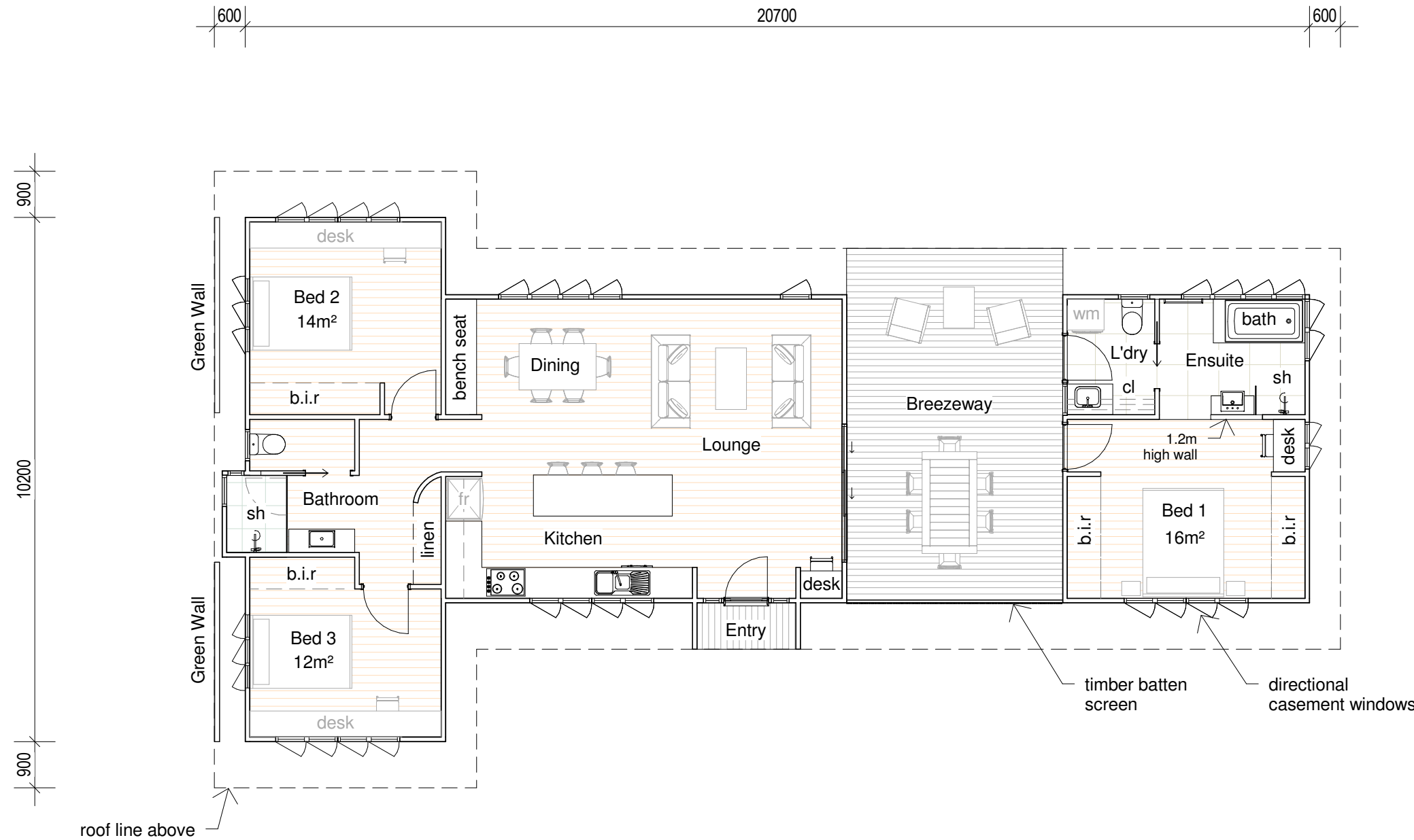
3 Bedroom 2 Bathroom Concept Design 1:100
