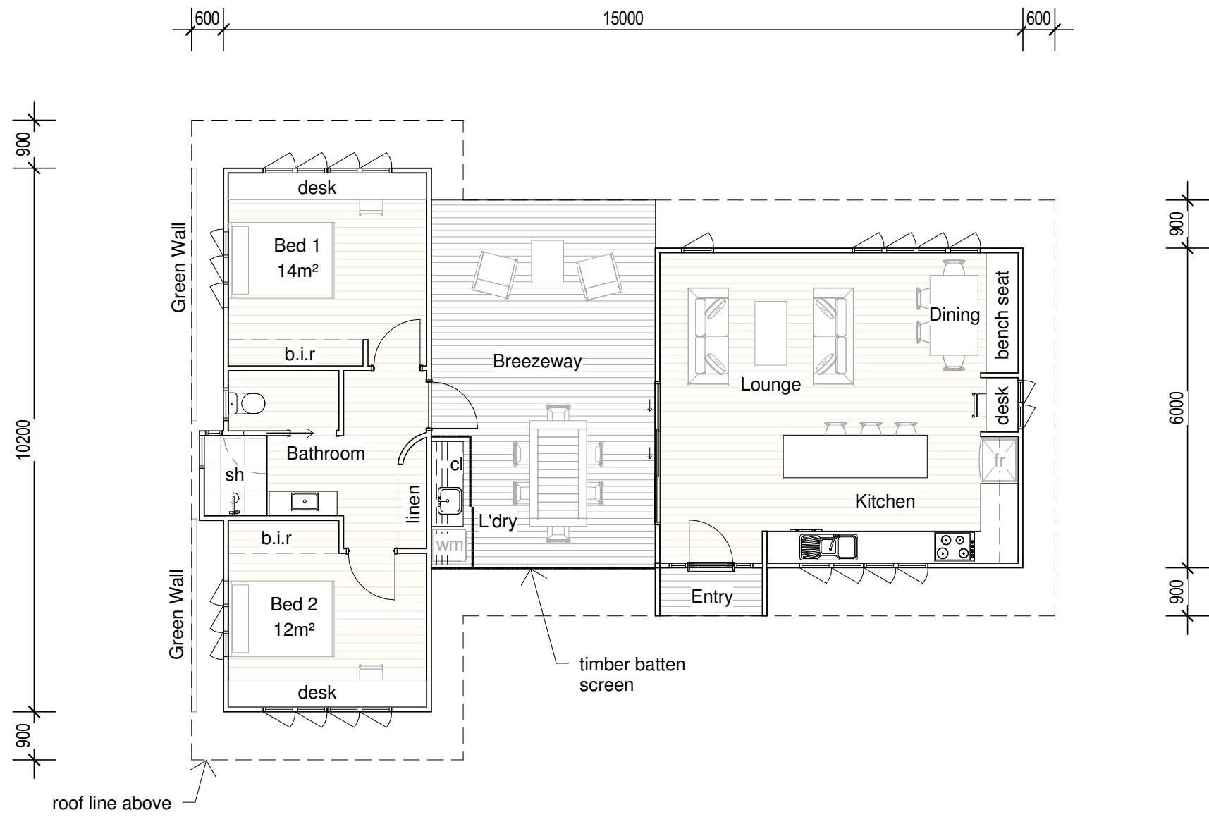
2 Bedroom 1 Bathroom Concept Design 1 : 100
